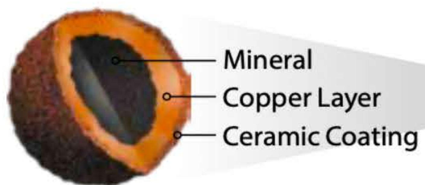
Illustration of a 3M copper roofing granule.
