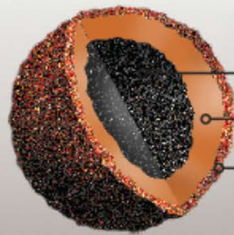
Illustration of a 3M copper roofing granule.
